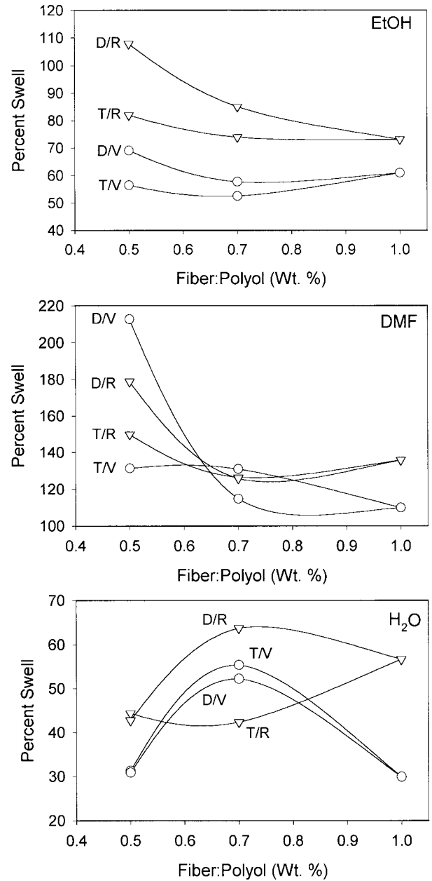
Figure 5 Effect of fiber-to-polyol ratio on the degree of swelling for polyurethane composites prepared with different fiber type and polyol functionality.
